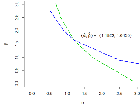
Figure 2: The plot of the ML estimates of \alpha and \beta graphically.
