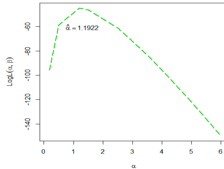
Figure 3: The curve of the log-likelihood function l(\alpha, \hat{\beta}) .
