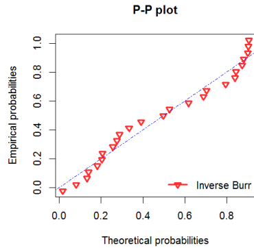
Figure 8: The P-P plot.
