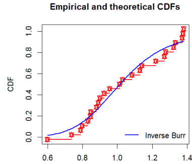
Figure 9: The CDF plot.
