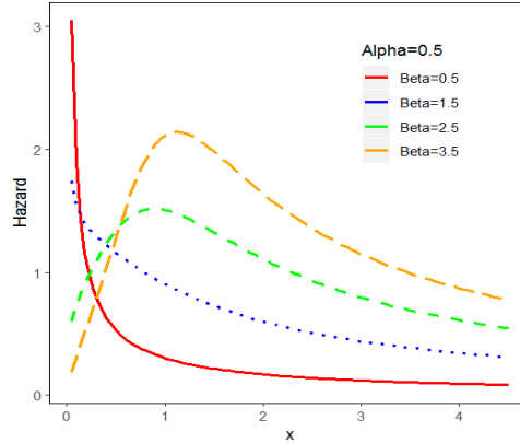
Figure 1: Graphs of the hazard rate function of the B-III distribution for different sets of parameters.
