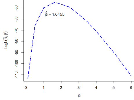
Figure 4: The curve of the the log-likelihood function l(\hat{\alpha}, \beta) .
