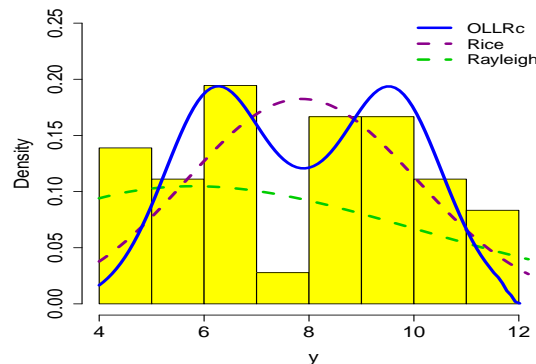
Figure 7: Estimated OLLRc, Rice and Rayleigh densities.
