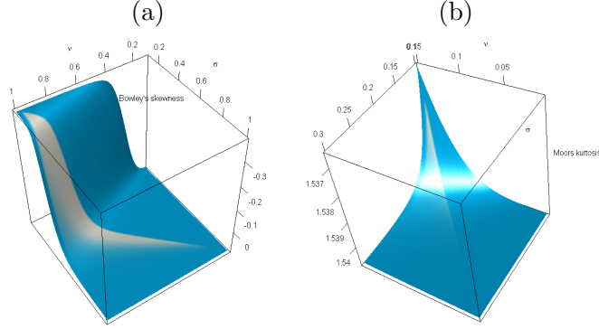
Figure 3: (a) Bowley's skewness. (b) Moors kurtosis.
