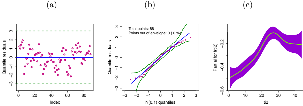
Figure 11: (a) Index plot of the qrs. (b) Normal probability plot for the qrs. (c) Smooth curve fitted from the OLLRc partially linear regression.
