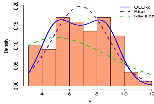
Figure 9: Estimated densities of the OLLRc, Rice and Rayleigh distributions.
