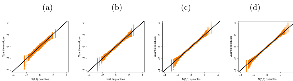
Figure 6: Normal probability plots of the qrs (scenario 1). (a) n = 60 . (b) n = 180 . (c) n = 400 . and (d) 700.
