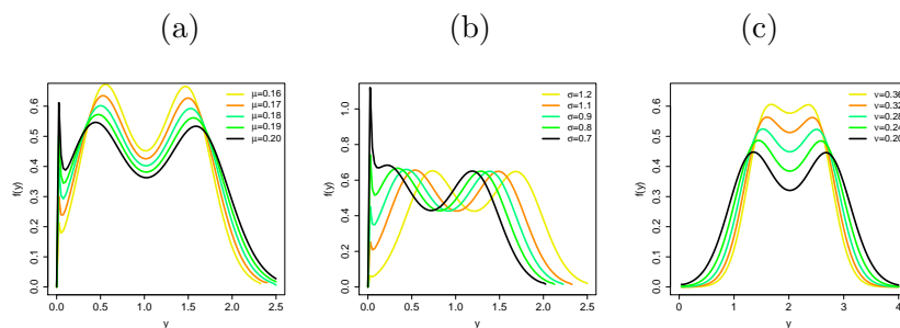
Figure 1: Plots of the OLLRc density. (a) For \sigma = 1 and \nu = 0.18 varying \mu . (b) For \mu = 0.16 and \nu = 0.17 varying \sigma . (c) For \mu = 0.25 and \sigma = 2 varying \nu .
