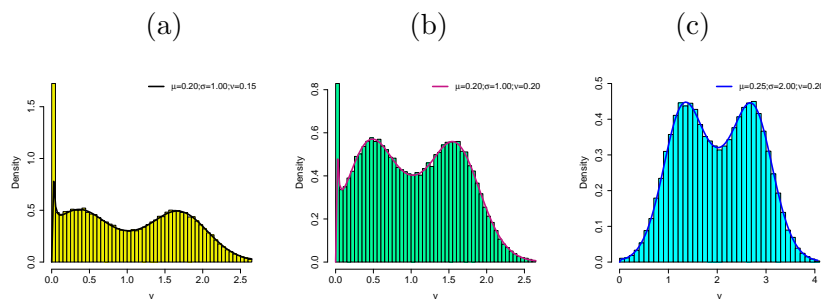
Figure 2: Histograms and plots of the OLLRc density.
