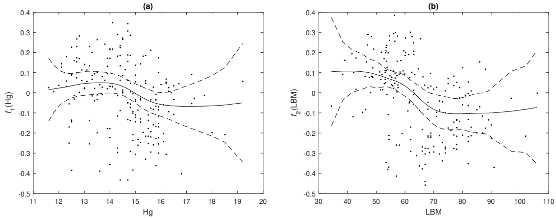
Figure 2: Plots estimated smooth functions f_1 (a) and f_2 (b) for the Australian athletes data and their approximate pointwise SEB denoted by the dashed lines.
