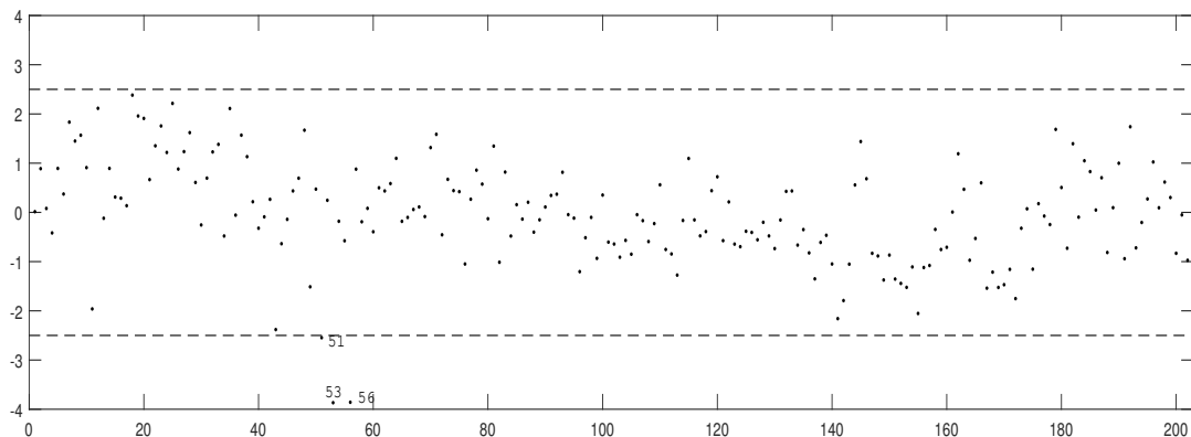
Figure 3: Plot standardized ordinary residuals versus the index of the observation.
