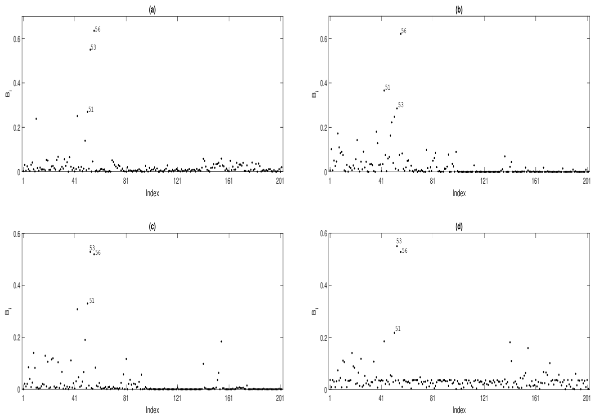
Figure 4: Index plots of B_i for assessing local influence on \hat{\boldsymbol{\beta}} (a), \hat{f}_1 (b), \hat{f}_2 (c) and \hat{\phi} (d) considering case-weight perturbation under model fitted to Australian athletes data.
