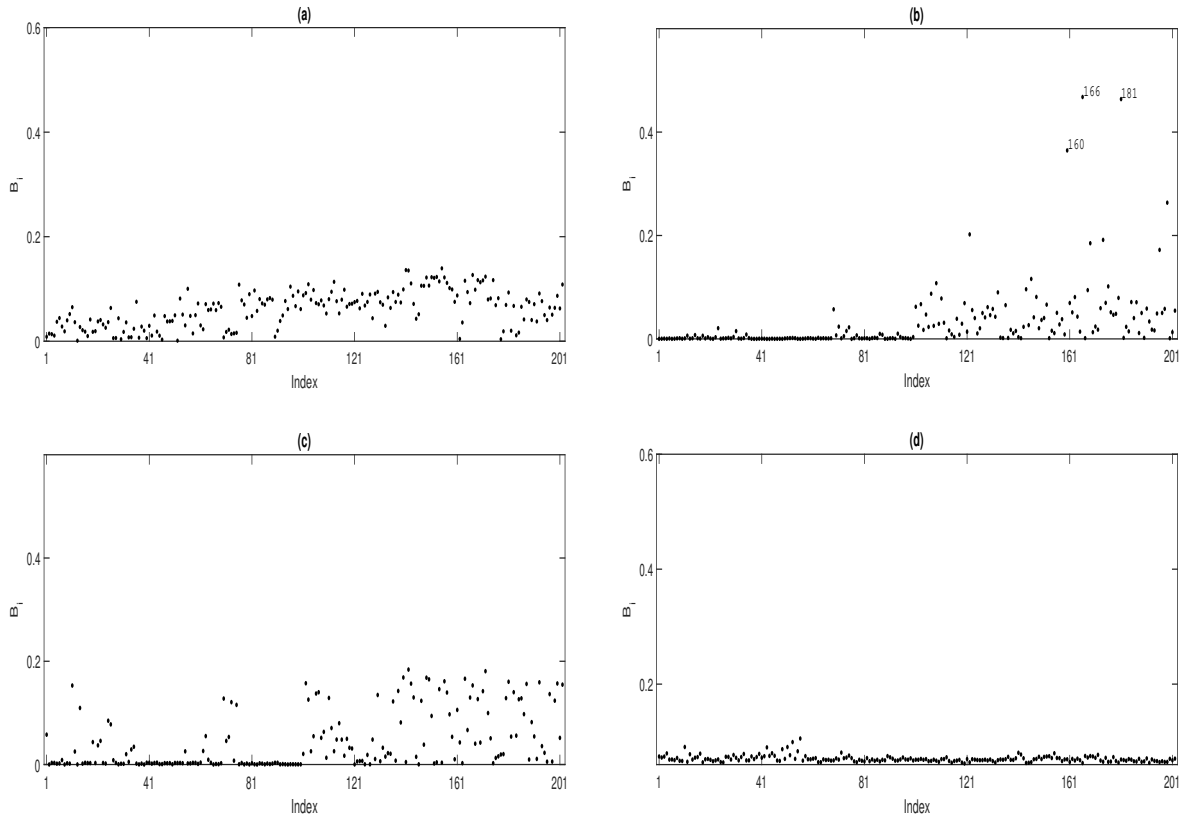
Figure 5: Index plots of B_i for assessing local influence on \hat{\beta} (a), \hat{f}_1 (b), \hat{f}_2 (c) and \hat{\phi} (d) considering response perturbation under the fitted model to Australian athletes data.
