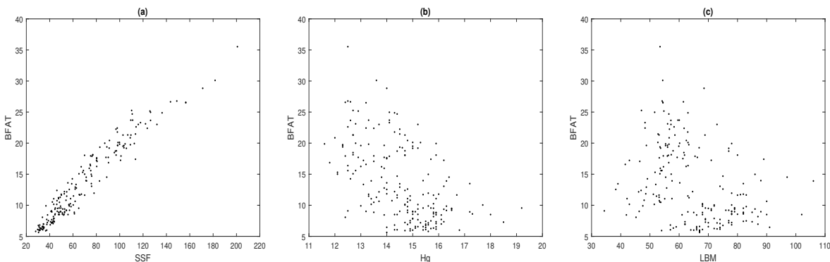
Figure 1: Scatter plots of BFAT versus SSF (a), HG (b) and LBM (c) with Australian athletes data.
