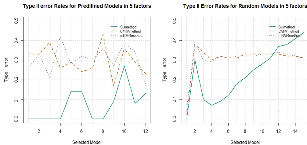
Figure 2: Comparisons of Type II error rates for Scenario A(left panel) and Scenario B (right panel) in case of five factor model. SU algorithm vs CMIM and mRMR.
