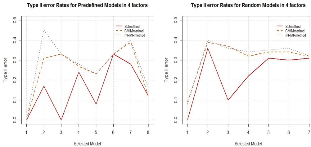
Figure 1: Comparisons of Type II error rates for Scenario A(left panel) and Scenario B (right panel) in case of four factor model. SU algorithm vs CMIM and mRMR (Scenario A).
