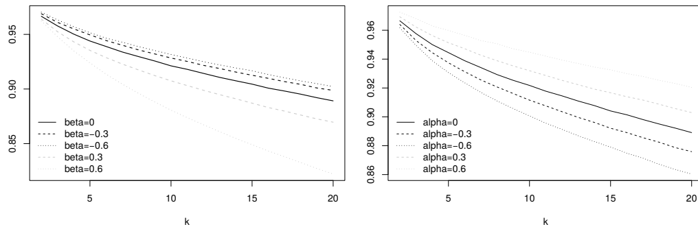
Figure 3: The probability of no signal up to the time point k for the EWMA control chart with \lambda = 0.1 and c = 2.04 . The target process is an ARFIMA(0,d,1) process with d = 0.2 (left side) and an ARFIMA(1,d,0) process with d = 0.2 (right side), respectively.
