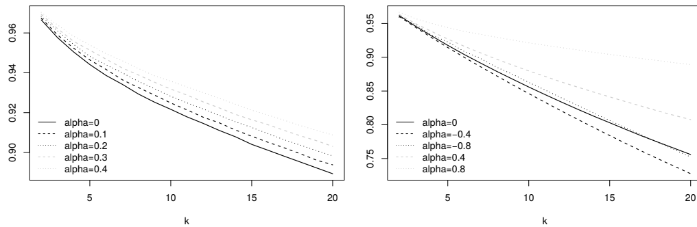
Figure 4: The probability of no signal up to the time point k for the EWMA control chart with \lambda = 0.1 and c = 2.04 . The target process is an ARFIMA(1,d,0) process with d = 0.2 (left side) and an ARFIMA(1,d,1) process with d = 0.2 and \beta = -0.8 (right side), respectively.
