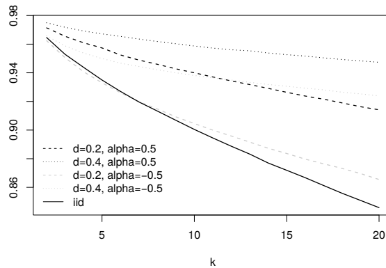
Figure 2: The probability of no signal up to the time point k for the modified EWMA chart with \lambda = 0.1 and c = 2.04 applied to an ARFIMA(1, d ,0) process.
