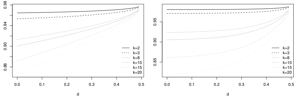
Figure 5: Probabilities of no signal up to the time point k as a function of d . The target process is an ARFIMA(0, d ,0) process. The EWMA parameters are c = 2.04 , \lambda = 0.1 (left), and c = 2.33 , \lambda = 1.0 (right).
