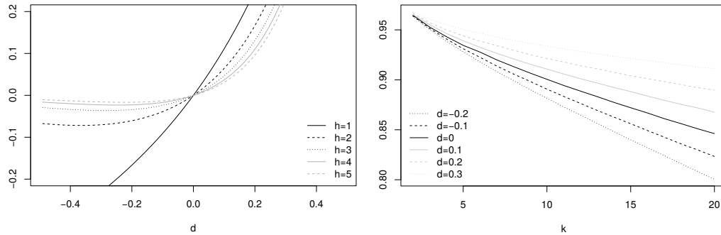
Figure 1: The first five autocorrelations \rho_d(h) (left side) and the probability of no signal up to the time point k (right side) for the modified EWMA chart with \lambda = 0.1 and c = 2.04 applied to an ARFIMA(0, d ,0) process.
